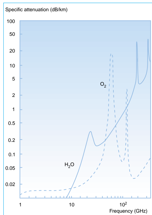
Figure 1 Specific attenuation due to atmospheric gases
