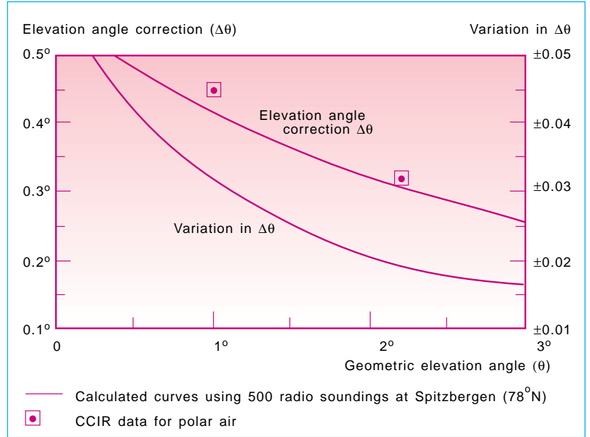
Figure 4 Average ray bending in polar areas
