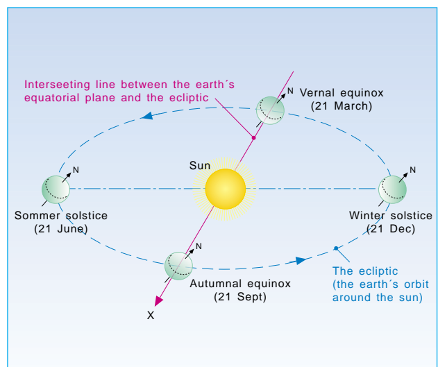
Figure 14 Definition of the x-axis in the geocentric equatorial coordinate system
