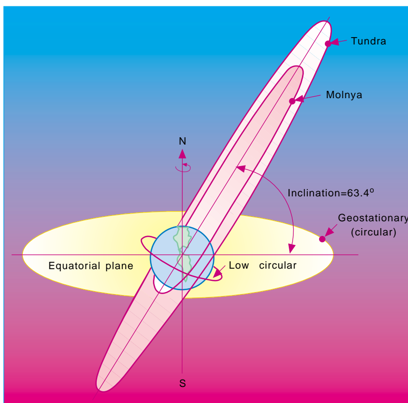
Figure 7 Different satellite orbits
