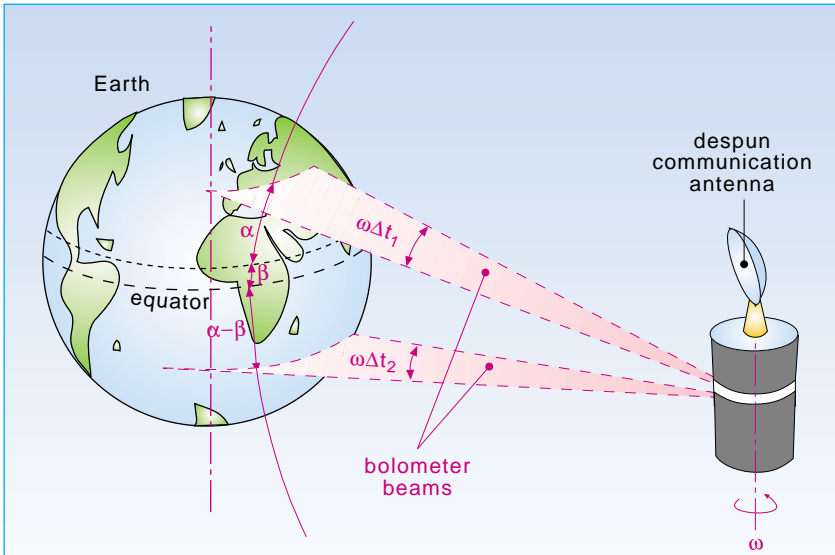
Figure 23 Earth contour detection by scanning infrared sensors (bolometers)
